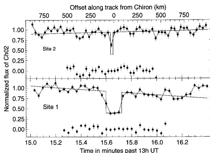
FIG. 4. Model fit for radius solution. The top graph shows the radius model fit superposed on the data from site 2, assuming that the single low point is due to an occultation chord. Below are the residuals to the fit. The bottom graph shows the fit, using the same model, to the site 1 data, where a nuclear chord was definitely observed.
