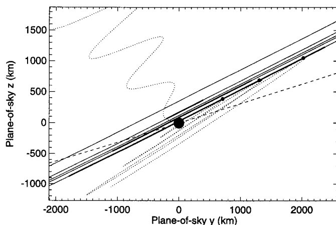
FIG. 6. Large area sky-plane geometry around Chiron. This plot is the same as Fig. 5 except for showing a larger region around Chiron. Only the tracks corresponding to the brighter component of Ch02 are shown and are not labeled for clarity. The heavy lines along these tracks mark the locations of the broad features, B1, B2, and B4. The filled circles mark the three most prominent minima in the periodic lightcurve structure. The orbit plane is indicated by the dashed line. Two spirals are drawn, depicting the geometry of two example dust jets. In this scenario, Chiron's pole is tipped 1^\circ out of the page, 33^\circ east of north (counter-clockwise). The ejection velocity is 36 \text{ m sec}^{-1} , the equatorial jet is aimed 6^\circ below the equatorial plane, and the polar jet is aimed 20^\circ away from the rotation axis.
