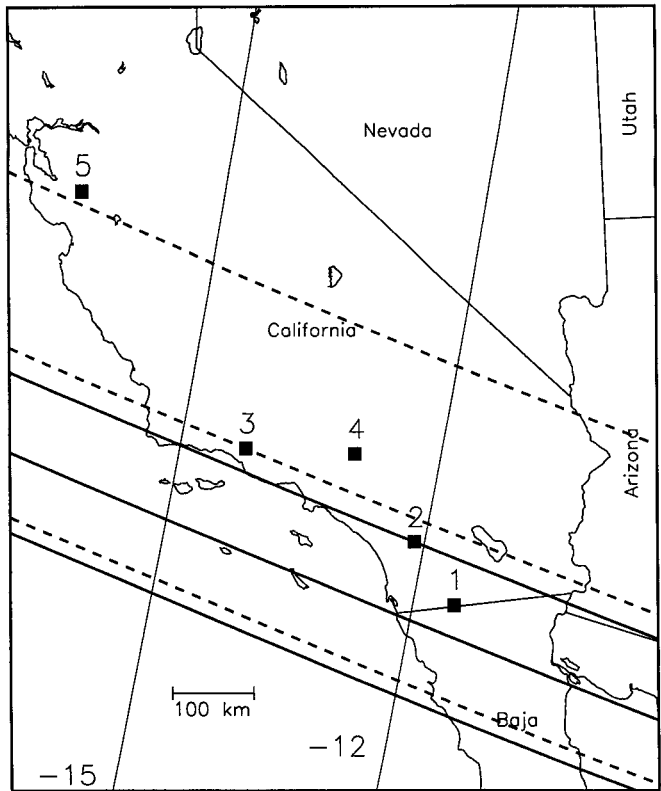
FIG. 1. Plot of the inferred shadow track of 2060 Chiron. The three dark lines running predominately east–west are the northern limit, centerline, and southern limit of Chiron's shadow, as inferred from the occultation results. The thinner, nearly north–south lines show the locations where the Sun elevation was -15^\circ and -12^\circ at 1993/11/07 13:15:30 UT, about the time Chiron's shadow crossed the coast. The dashed lines show the final predicted centerline and the \pm 1\sigma centerlines for the occultation, determined from the strip-scan astrometry. The locations of the five observing sites are indicated by square symbols.
