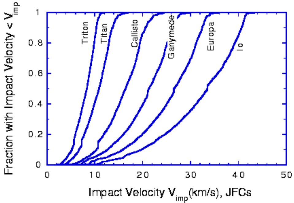
Figure 4. Cumulative impact velocity distributions for impacts by ecliptic comets on various satellites in the solar system. These are the result of a Monte Carlo simulation; the occasional unsightly glitches are caused by rare objects in orbits with very high impact probability.
