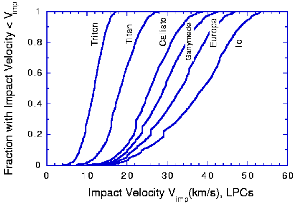
Figure 6. Cumulative impact velocity distributions for impacts by long period or Halley-type comets on various satellites in the solar system.
