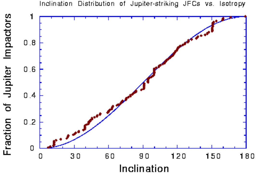
Figure 2. The cumulative jovicentric inclination distribution of the 144 test particles that hit Jupiter in LD97. This is compared to the isotropic distribution.
