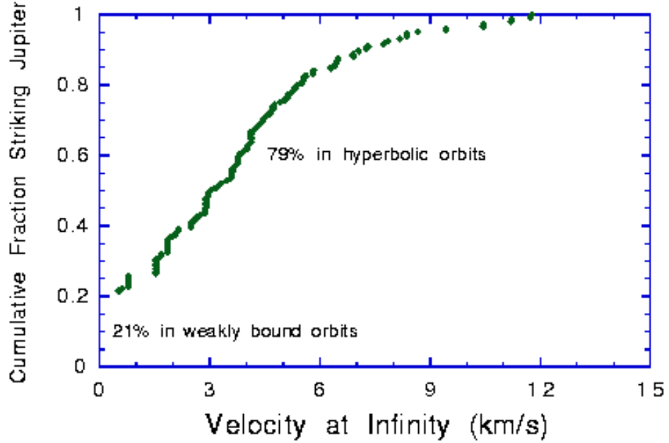
Figure 1. The cumulative distribution of encounter velocities ( v_\infty ) with Jupiter (velocities at infinity) for the 144 objects striking Jupiter in LD97. The objects plotted at v_\infty = 0 were orbiting Jupiter when they struck the planet; these are 21% of the total.
